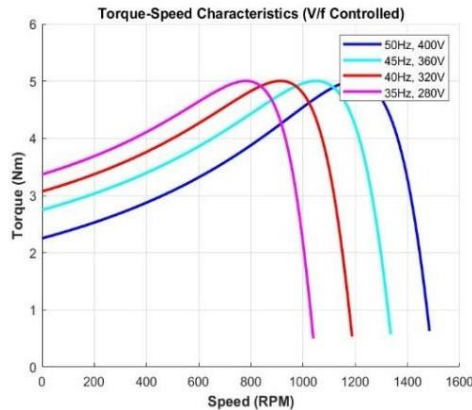
Figure.6 Torque Vs Speed Curves
