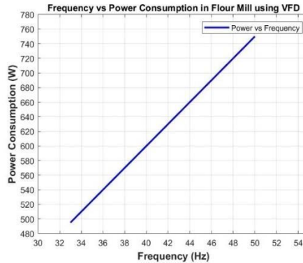
Figure.8 Frequency vs Power Consumption
